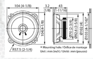
KFC-S1056 PEAK POWER 220W RMS POWER 21W
