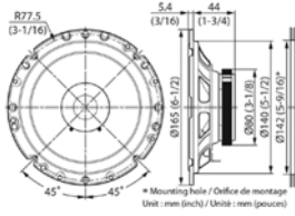
KFC-S1756 PEAK POWER 300W RMS POWER 30W
