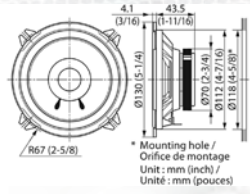
KFC-S1356 PEAK POWER 260W RMS POWER 30W
